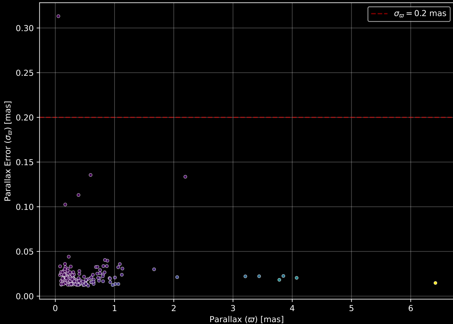
APOGEE DR17 Field: [229-04] Parallax Quality (n= 182)
