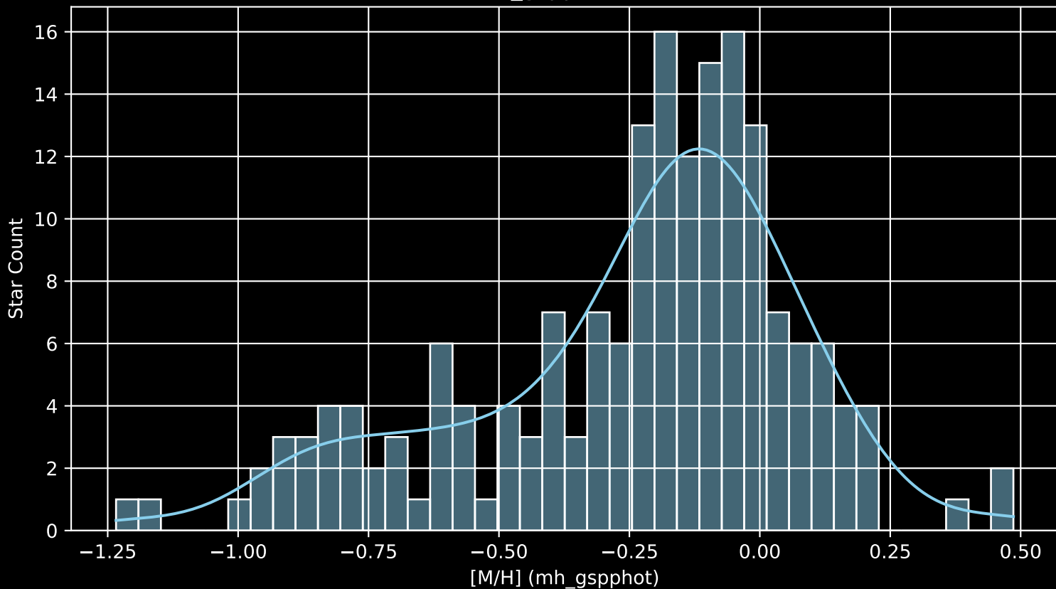
APOGEE DR17 Field: [229-04 [M/H] (mh_gspphot) (n= 181)
