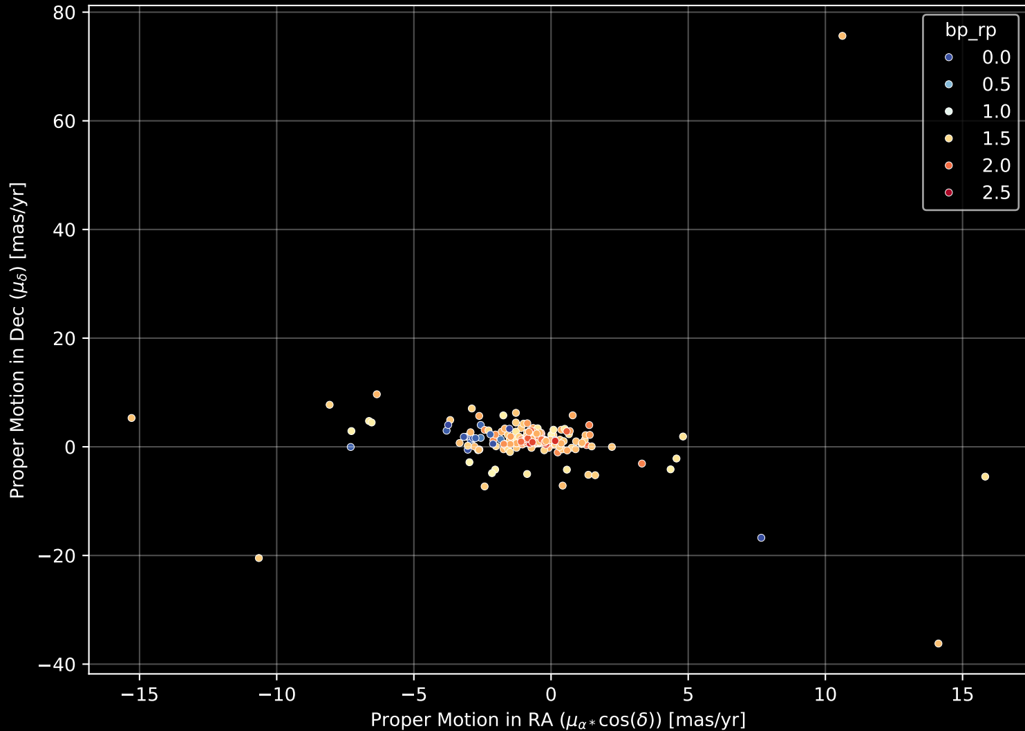
APOGEE DR17 Field: [229-04] Proper Motion Diagram (n= 182)
