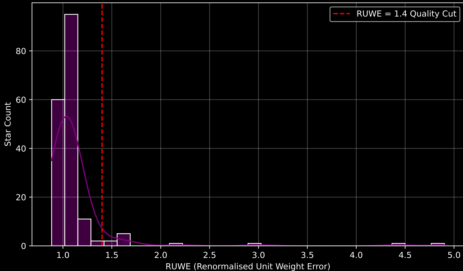
GAPOGEE DR17 Field [229-04] RUWE Distribution (n= 179)
