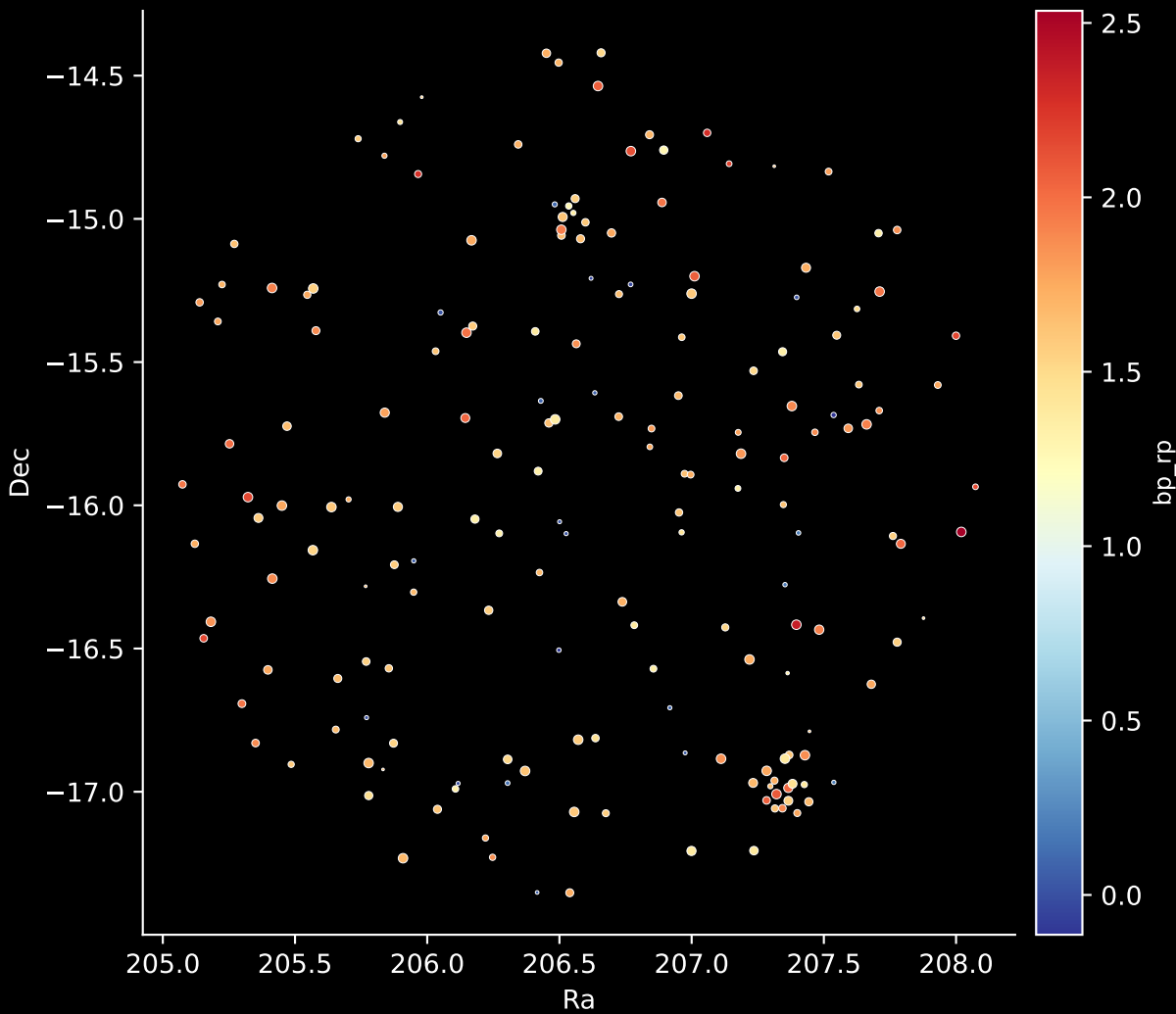
APOGEE DR17 Field: [229-04] Stars: 182
